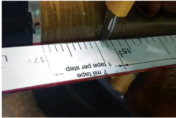
Template for insulation stepping is designed for specific cable and provided in the joint kit.
