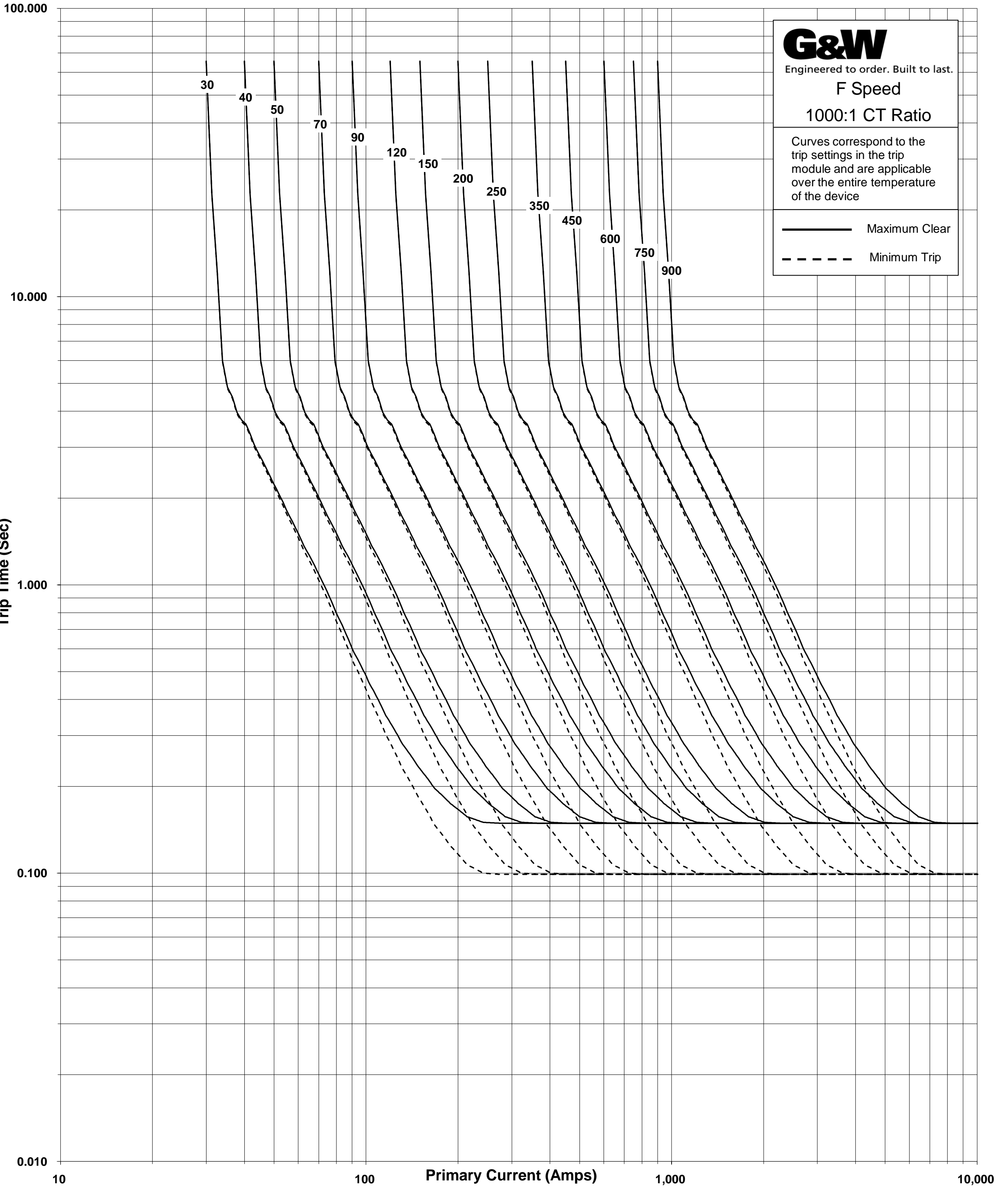
TIME - CURRENT CHARACTERISTIC CURVES FOR VI CONTROLS
