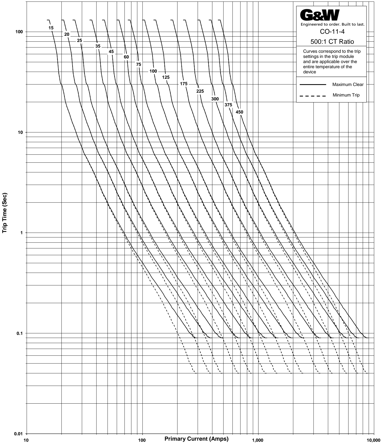
TIME - CURRENT CHARACTERISTIC CURVES FOR VI CONTROLS
